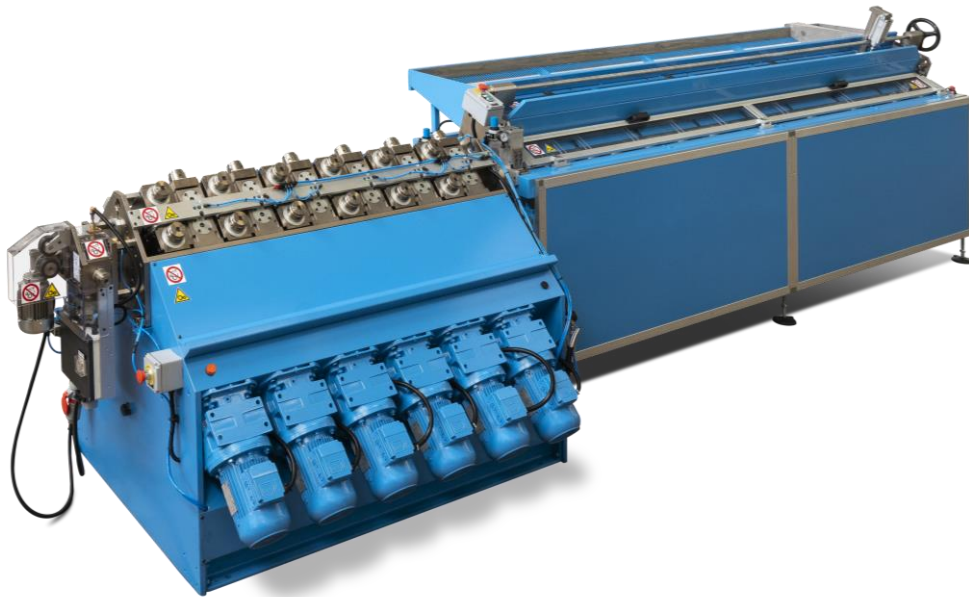
Figure 1 Roll reducing mill with 12-station rolls with unloading device.
